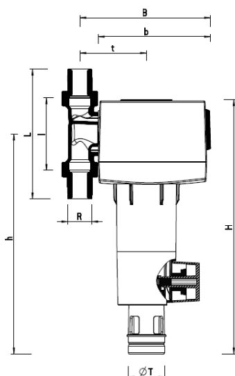
Figure 3: Dimensions of Logafix water filter with connector
